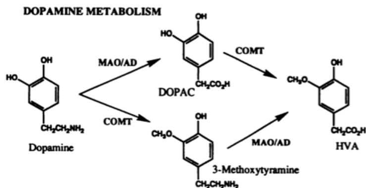
Figure 9: Dopamine metabolism - Multistep pathway in the central nervous system. Abbreviations: COMT: catechol-O-methyltransferase; DOPAC: dihydroxyphenylacetic acid; HVA: homovanillic acid; MAO/AD: monoamine oxidase/aldehyde dehydrogenase. Adapted from Volkow et al, 1996
