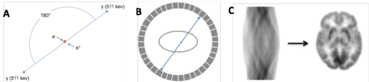
Figure 28: PET Principle - (A) Annihilation reaction (B) Detection of coincidences (C) Reconstruction from the sinogram. Adapted with permission from Ines Merida
