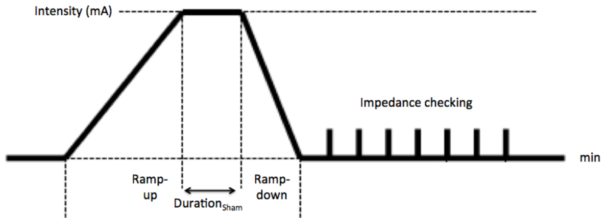
Figure 17: Sham tDCS waveform. Adapted from NeuroConn Manual
