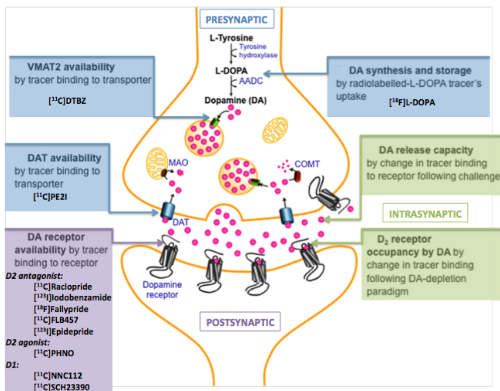
Figure 25: Dopaminergic imaging targets and PET radiotracers - Most common PET radiotracers to assess the dopaminergic system in the presynaptic and post-synaptic compartments. Adapted from Weinstein et al., 2017
